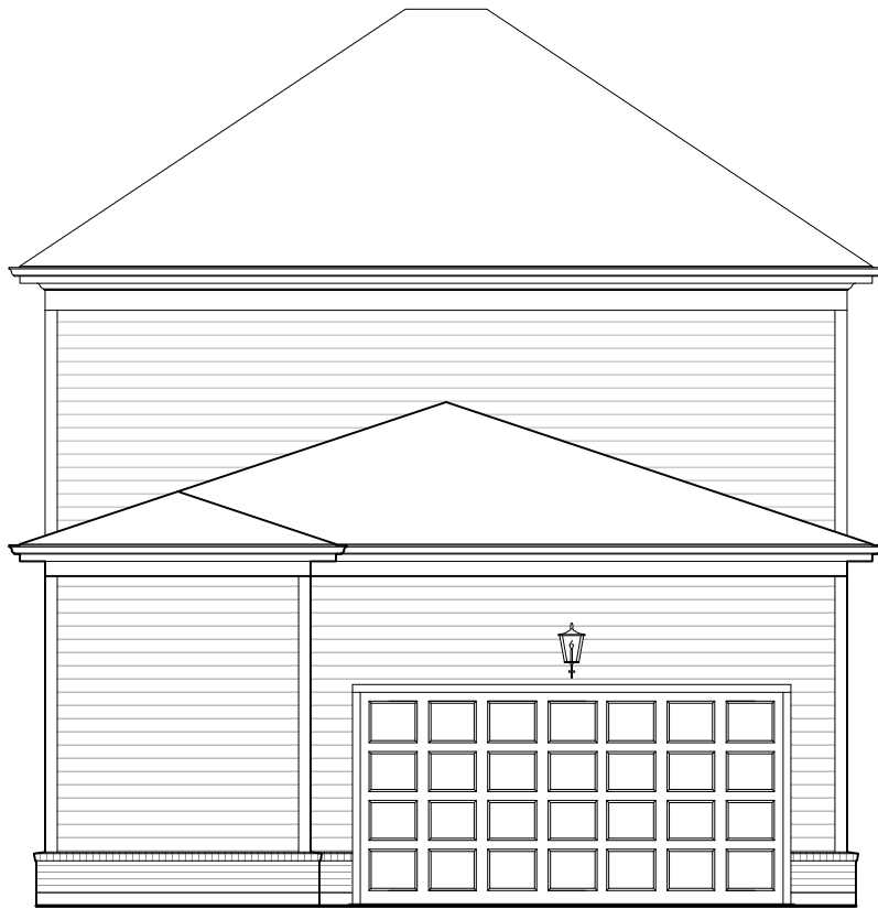
REAR ELEVATION
