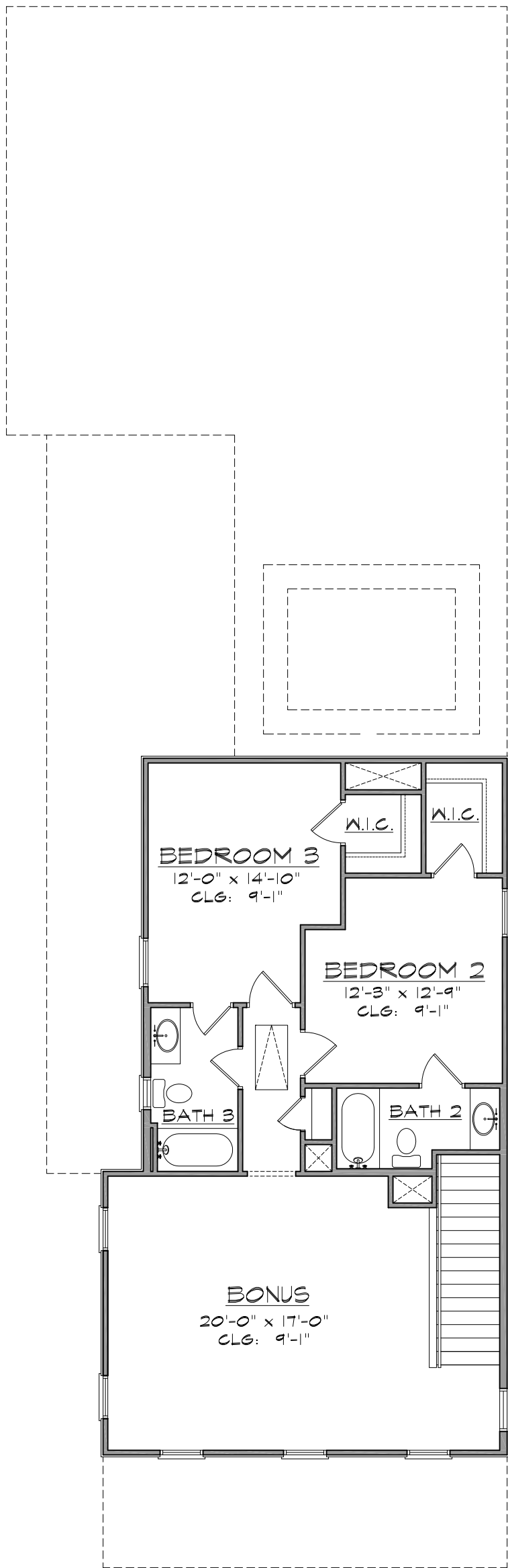
UPPER LEVEL FLOOR PLAN
