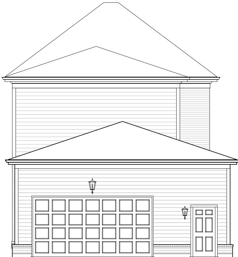
REAR ELEVATION
