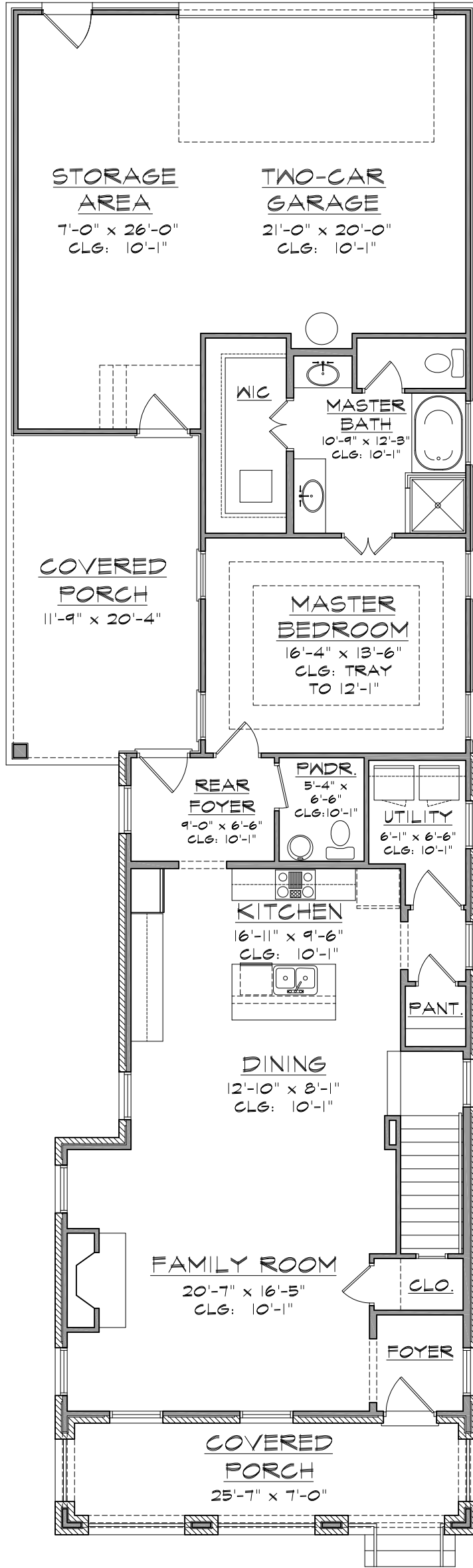
MAIN LEVEL FLOOR PLAN
